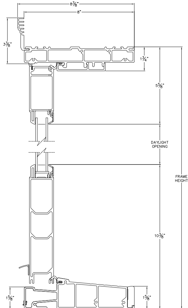
HEAD & SILL
