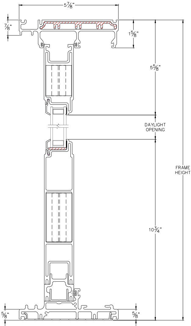
HEAD & SILL
