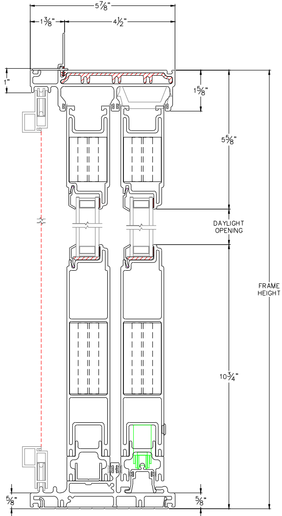
HEAD & SILL
