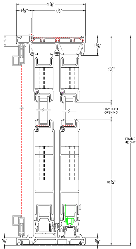
HEAD & SILL
