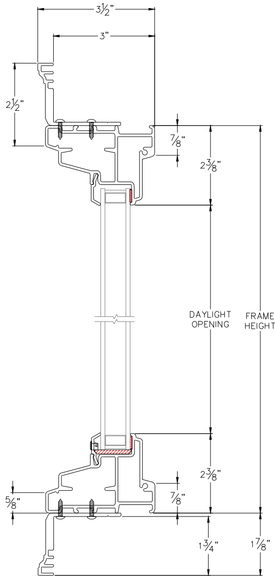
HEAD & SILL
