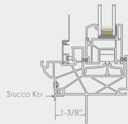
1 3/8" MOUNTING FIN SET-BACK W/ STUCCO KEY*
