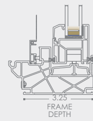
3.25 FRAME DEPTH
